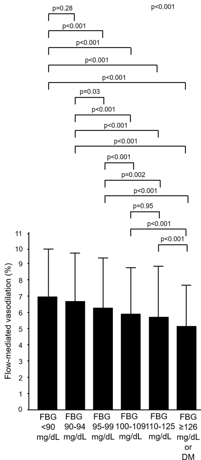
Figure 1 Bar graphs show flow-mediated vasodilation in subjects with FBG of <90, 90–94, 95–99, 100–109, 110–125, and ≥126 mg/dL or known diabetes. DM, diabetes mellitus; FBG, fasting blood glucose.
